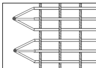
Welded into groups of 3
